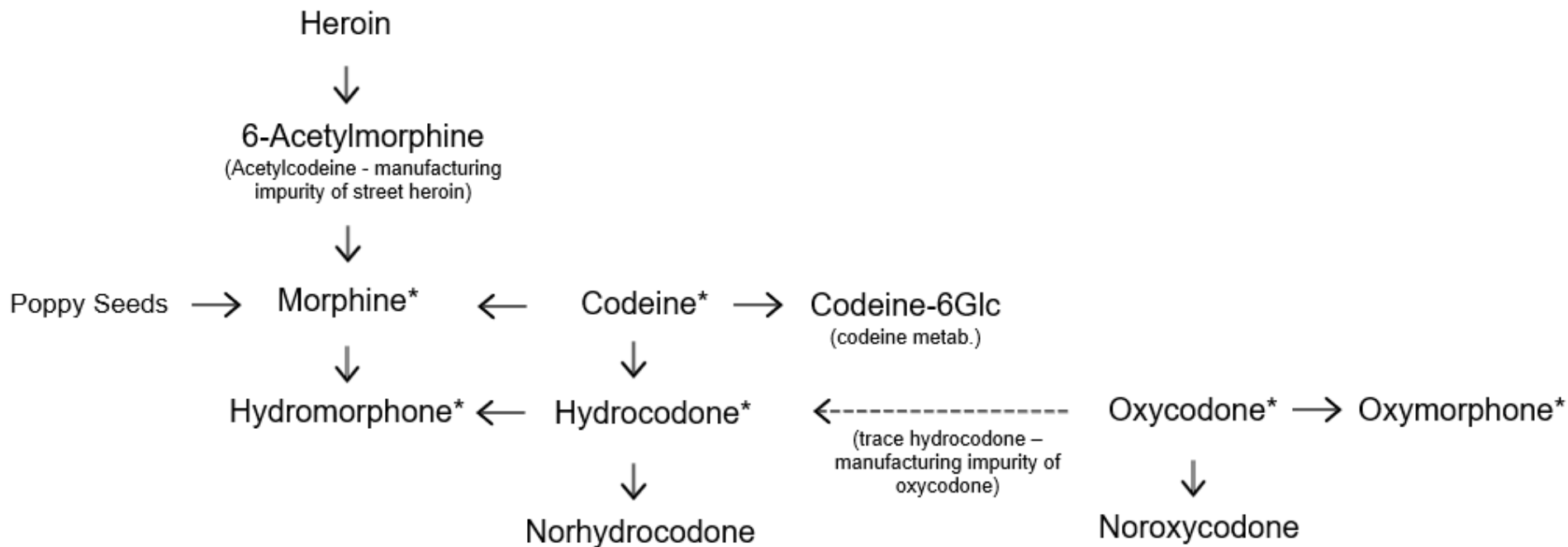
Figure 1. Principal Opiate Metabolic Pathways
