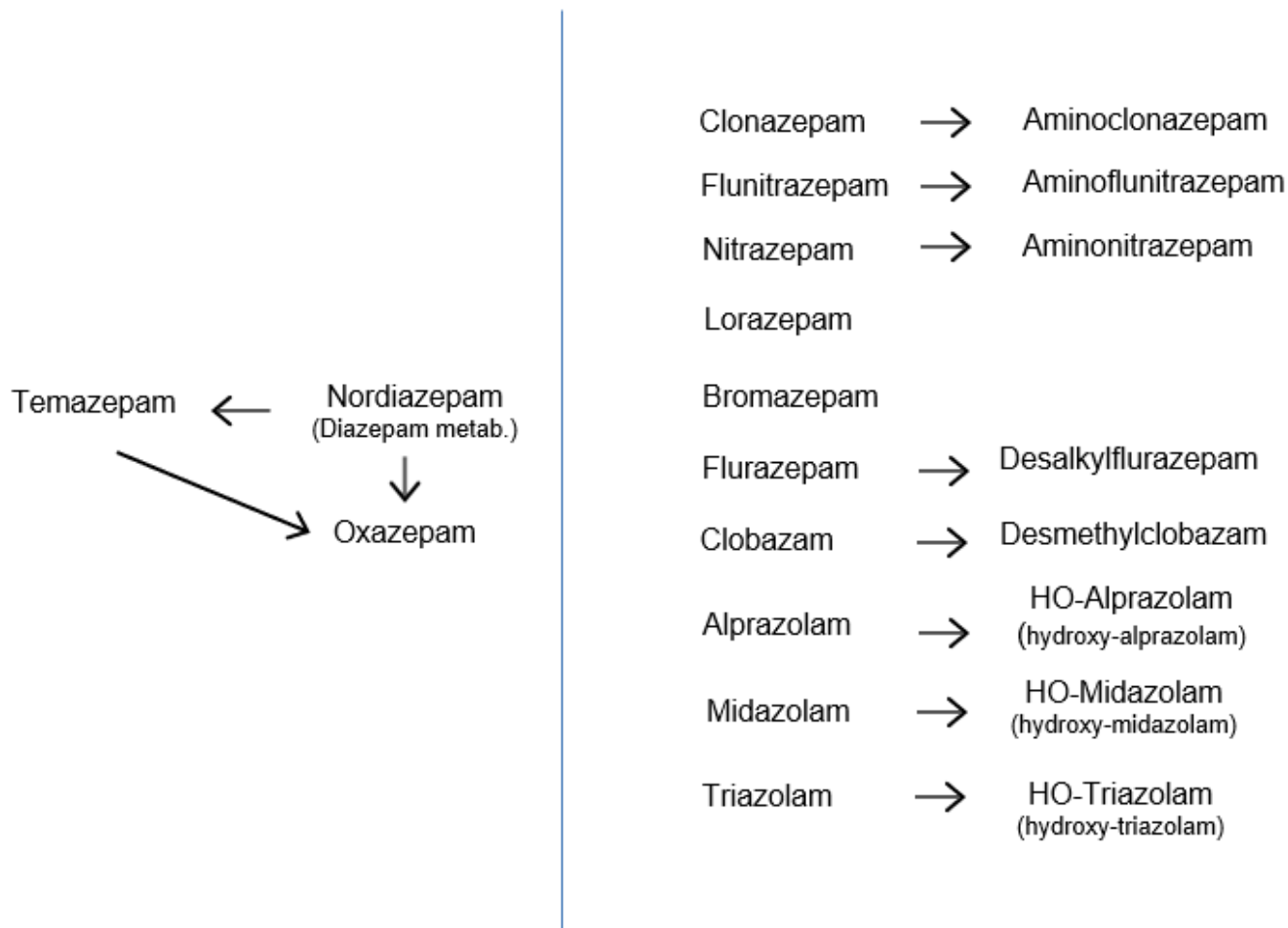
Figure 2. Principal Benzodiazepine Metabolic Pathways
